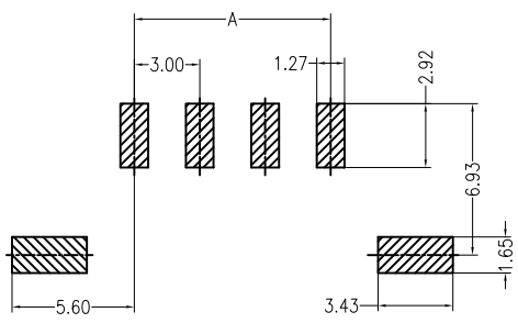
PCB LAYOUT(Tolerance:±0.05)
